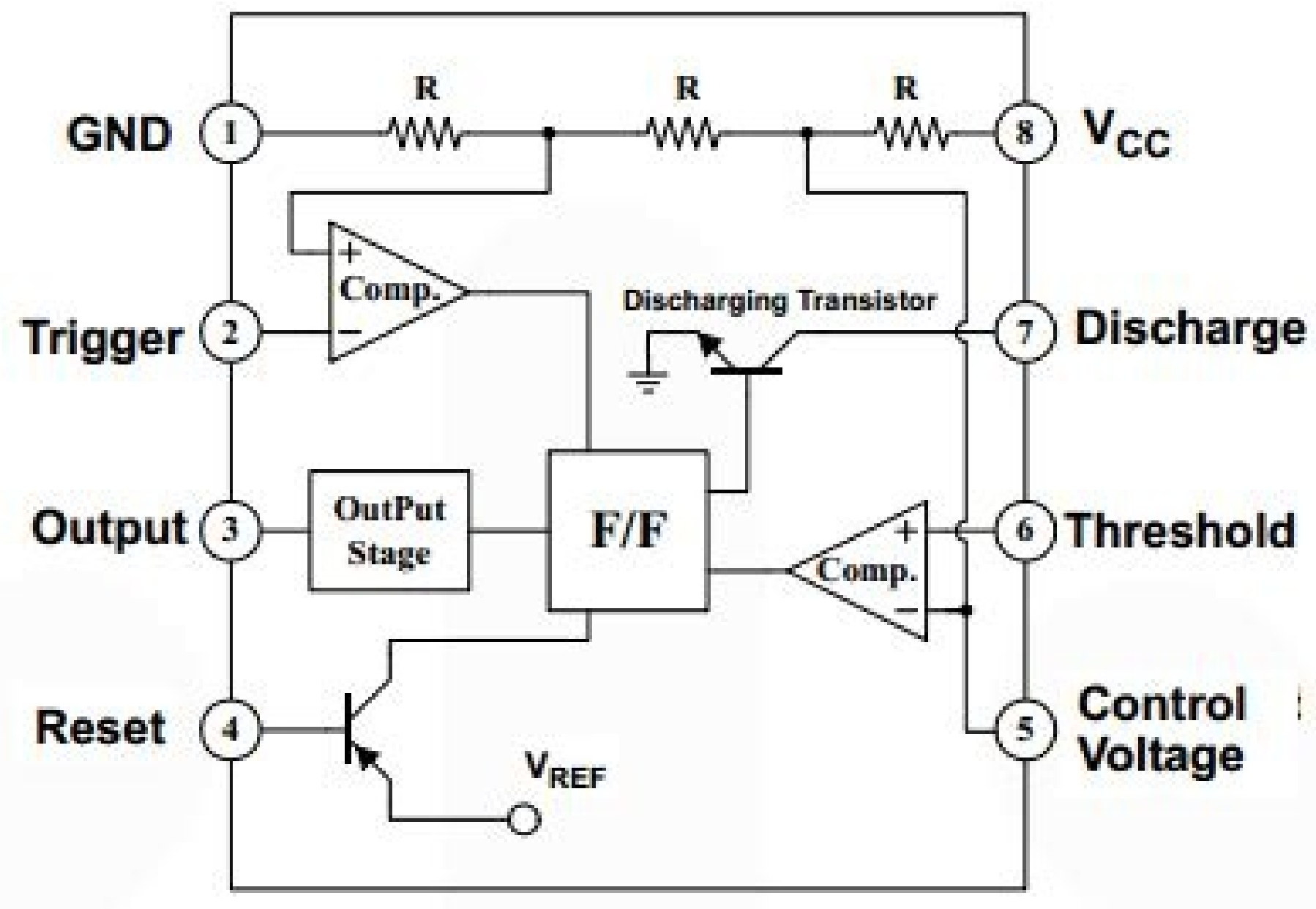
Figure 1. Block Diagram
